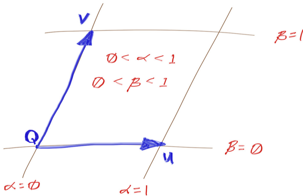
Figure 7: Quadrilateral coordinates
