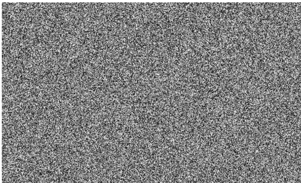
Image 6: White noise
