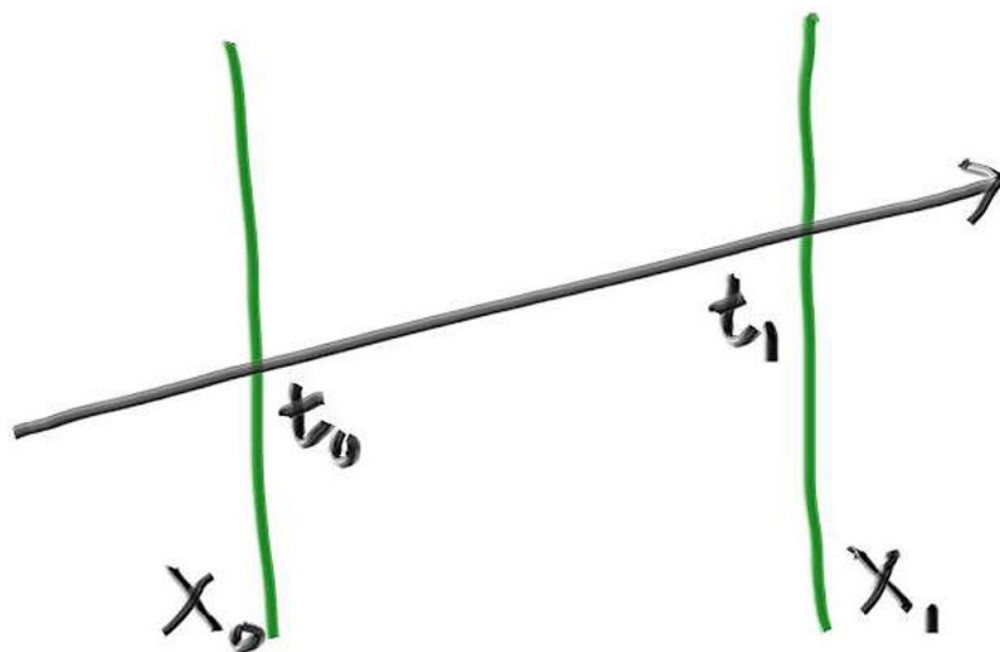
Figure 3: Ray-slab intersection
