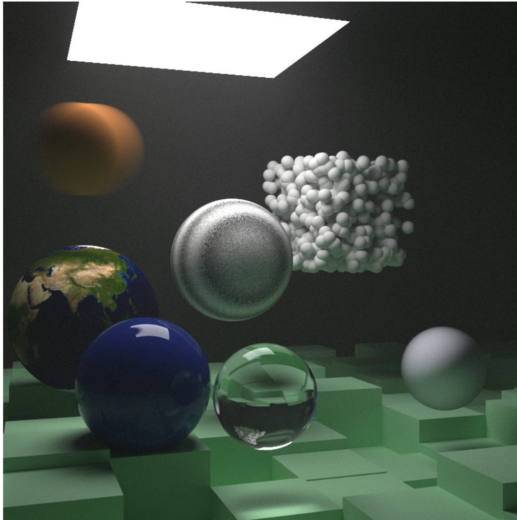
Image 23: Final scene
