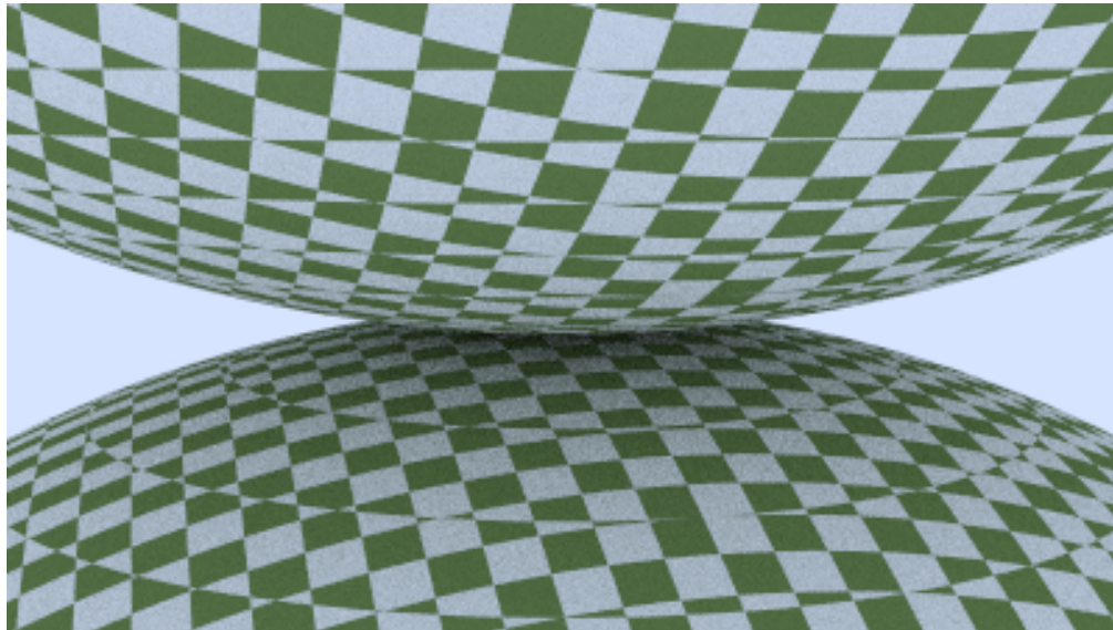
Image 3: Checkered spheres
