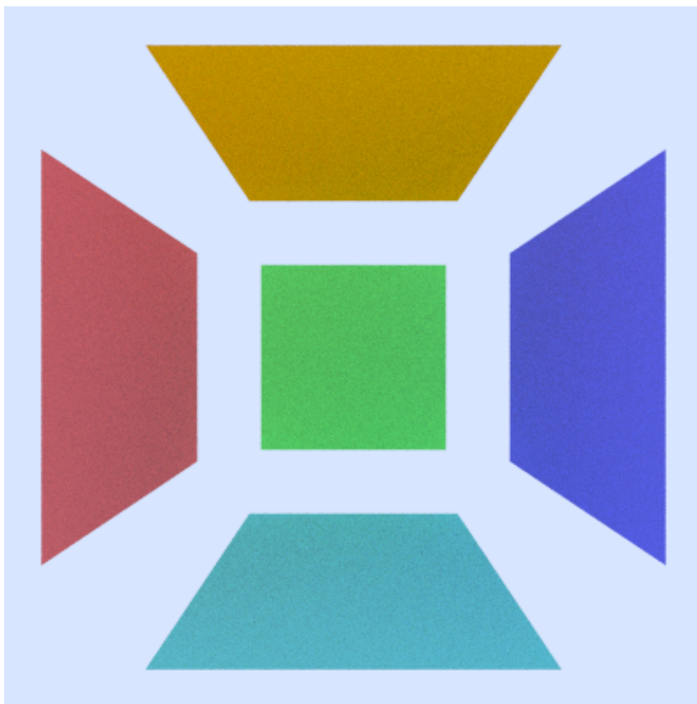
Image 16: Quads
