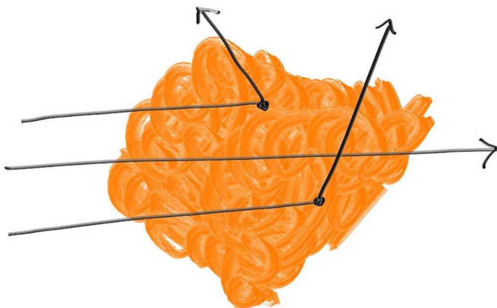
Figure 10: Ray-volume interaction
