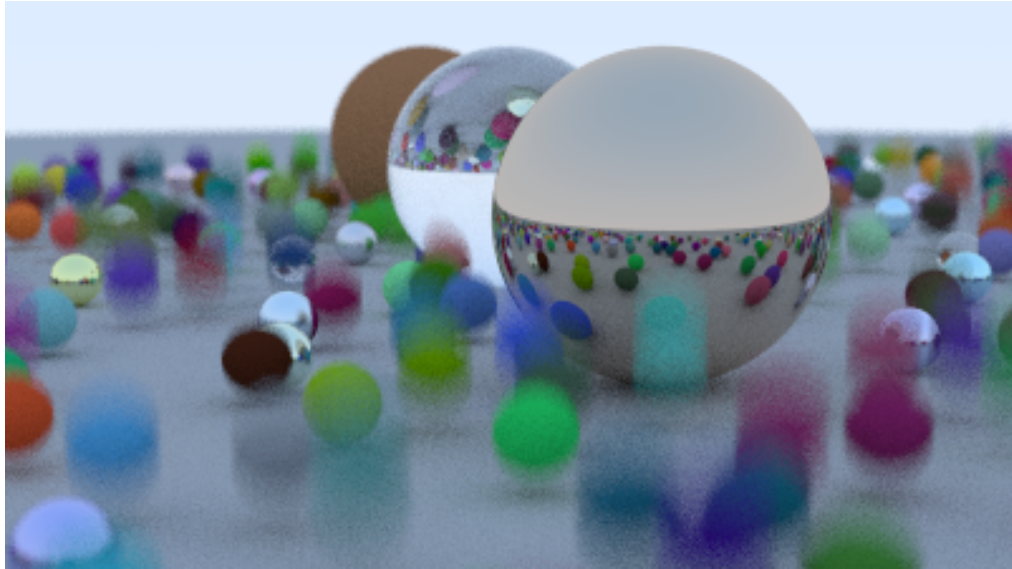
Image 1: Bouncing spheres
