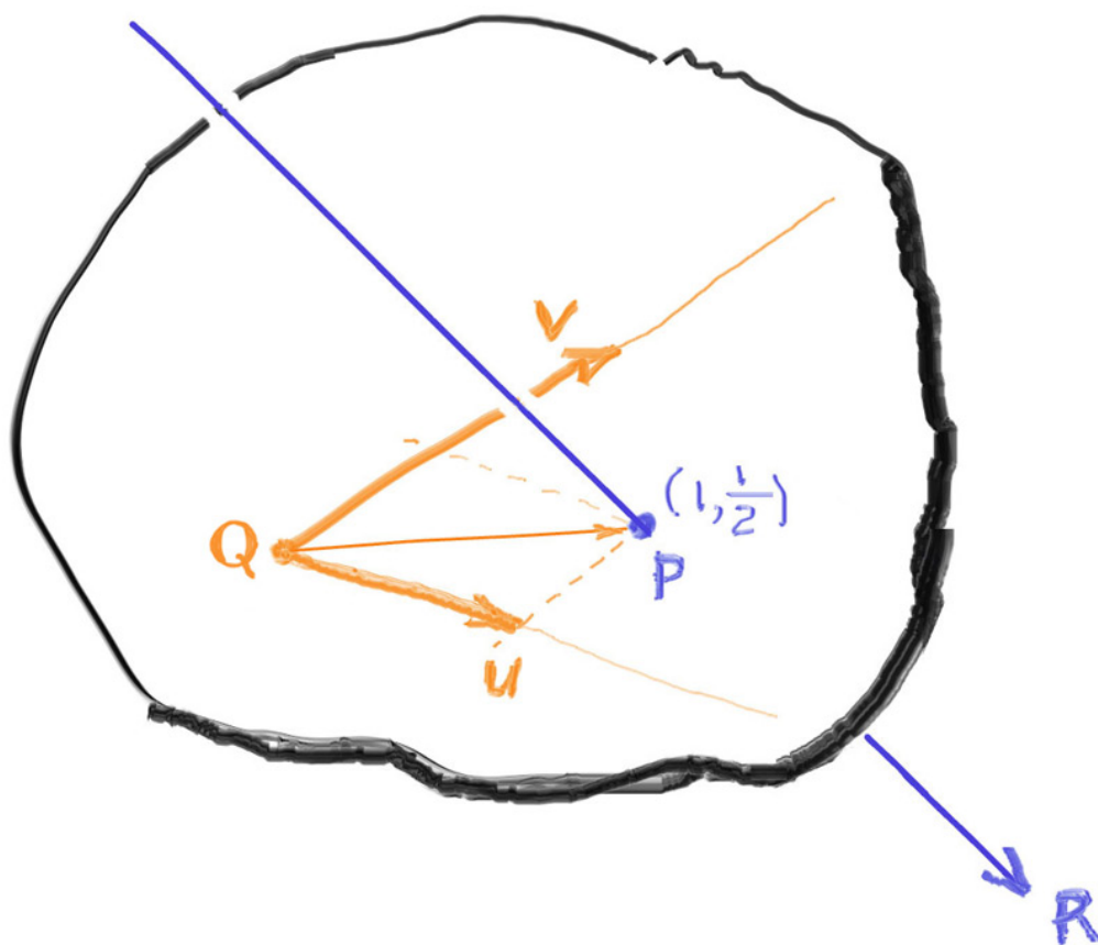
Figure 6: Ray-plane intersection
