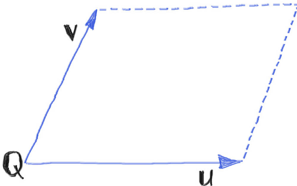
Figure 5: Quadrilateral Components
